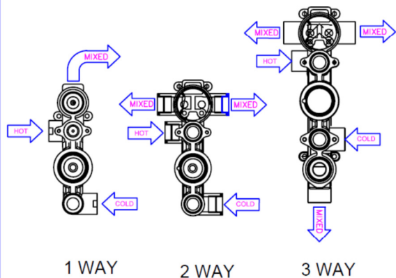
Fig3: CONNECT WATER OUTLETS
